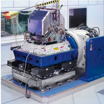
Philae on the 200 kN shaker
