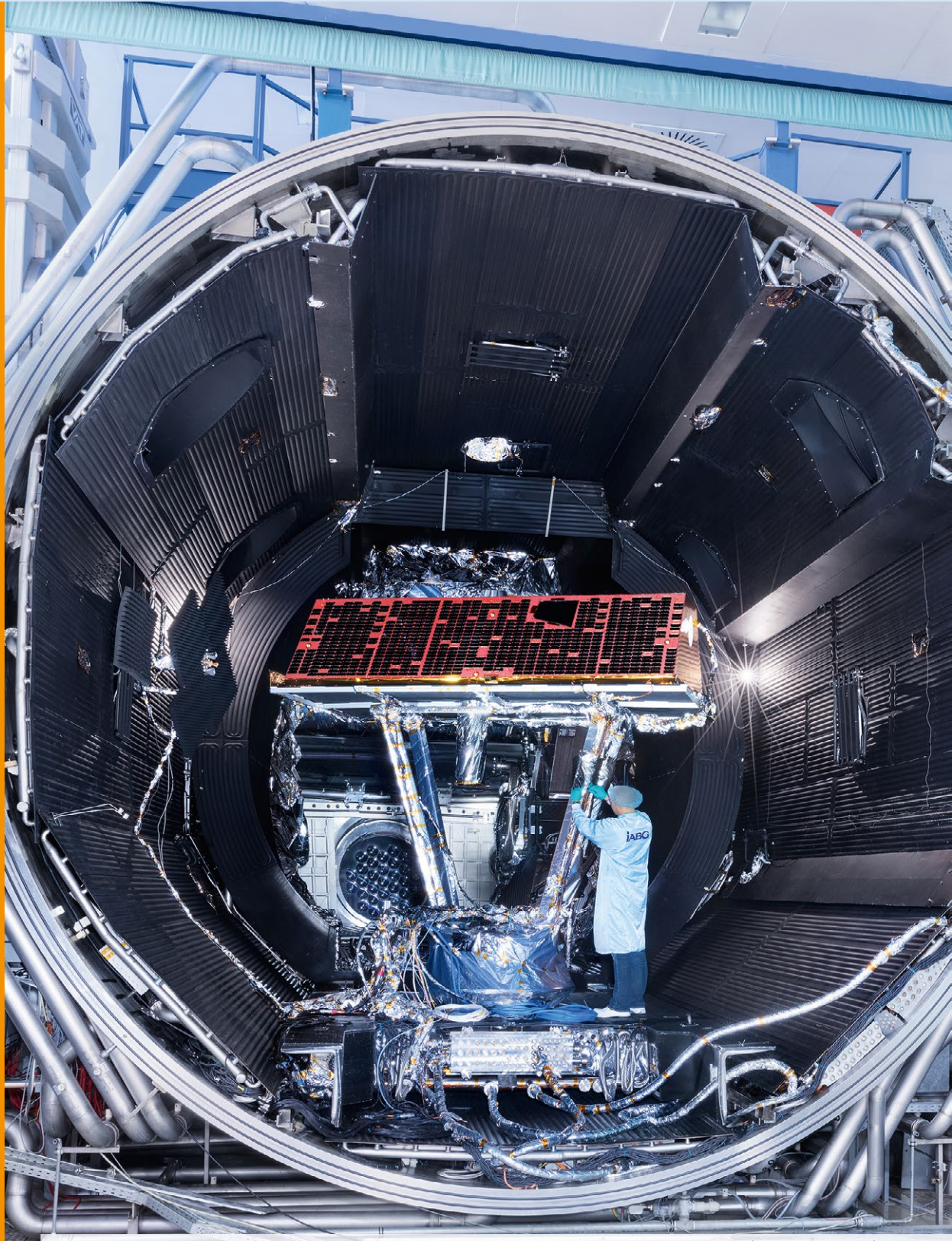
The Gravity Recovery and Climate Experiment-Follow-On (GRACE-FO) in Space Simulation Chamber • Airbus Defence and Space is the prime contractor for GRACE-FO
