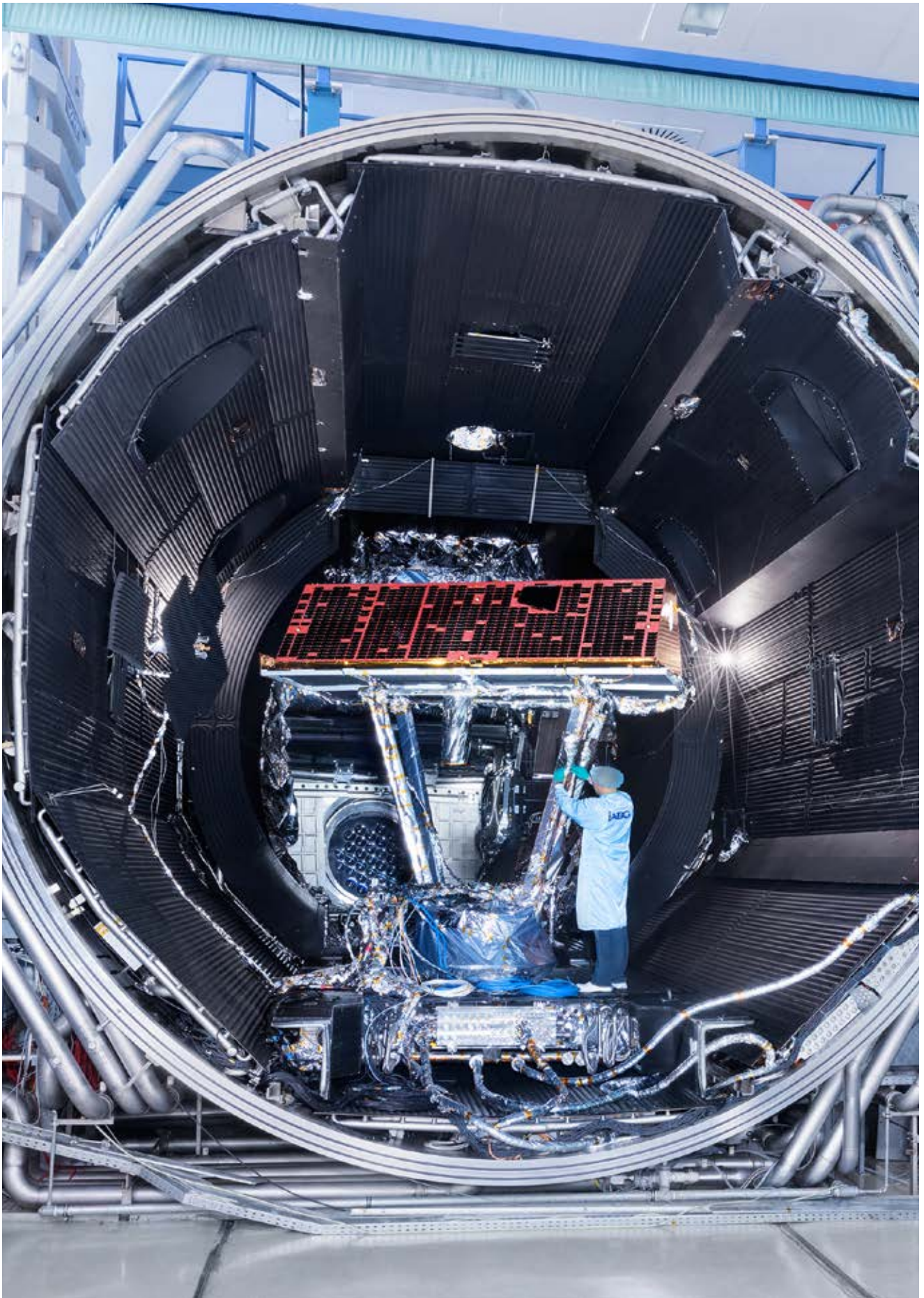
The Gravity Recovery and Climate Experiment-Follow-On (GRACE-FO) the space simulation chamber Airbus Defence and Space is the prime contractor for GRACE-FO
